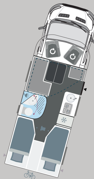
Challenger 287 GA L/B/H: 6,99m / 2,35m / 2,92m
